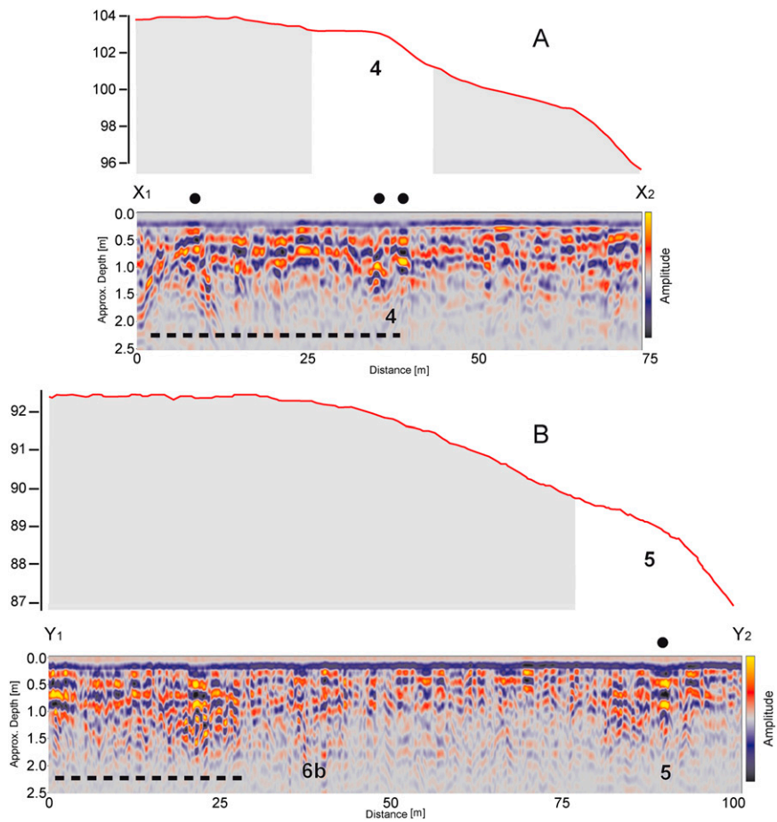
Fig. S5. LiDAR-derived topographic profiles and GPR 2D profiles X_1 - X_2 (A) and Y_1 - Y_2 (B) acquired on the top and southeast sector (grid 2) of Mt. San Rocco, respectively (for the location, see Fig. S3). Black dots mark possible walls; dotted lines show the areas where archeological structures are more apparent; bold numbers highlight the position of archeological structures shown in Figs. S3 and S4.
